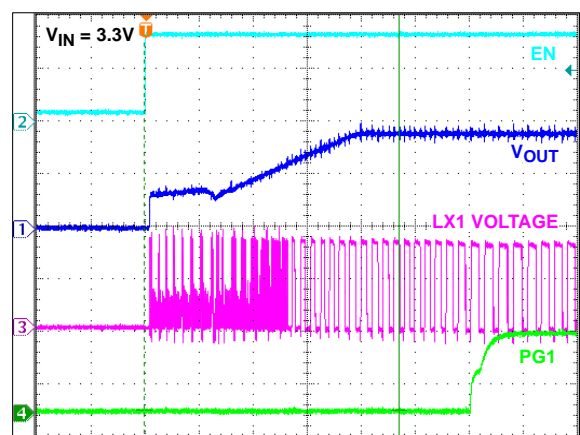
FIGURE 46. SOFT-START AT 6A LOAD
