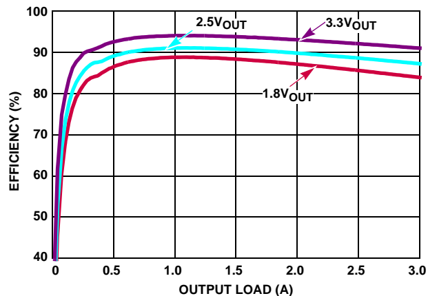
FIGURE 6. EFFICIENCY, V_{IN} = 5\text{V} , T_A = +25^\circ\text{C}
