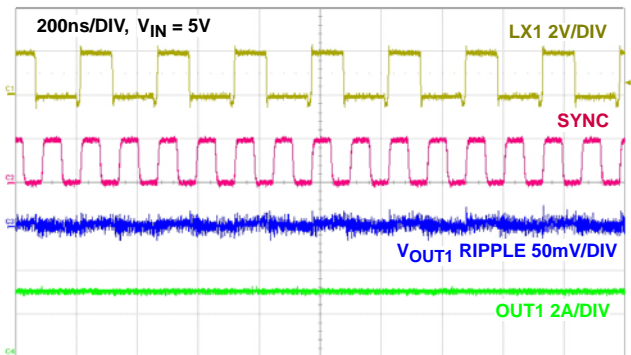
FIGURE 25. STEADY STATE OPERATION CHANNEL1 3A LOAD WITH F_{SW} = 4\text{MHz}
