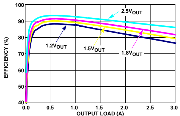
FIGURE 2. EFFICIENCY vs LOAD CURRENT, V_{IN} = 3.3V , T_A = +25^\circ C
