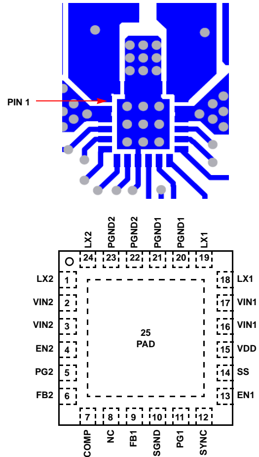
FIGURE 52. RECOMMENDED THERMAL PAD LAYOUT
