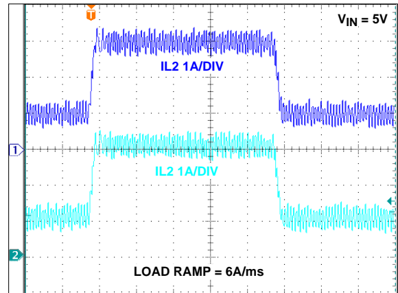
FIGURE 48. CURRENT SHARE BALANCING, 2A TO 6A
