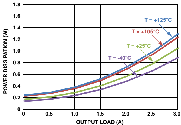
FIGURE 8. POWER DISSIPATION, V_{IN} = 5\text{V} , V_{OUT} = 1.8\text{V}
