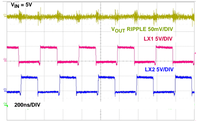
FIGURE 42. STEADY STATE OPERATION AT 6A LOAD
