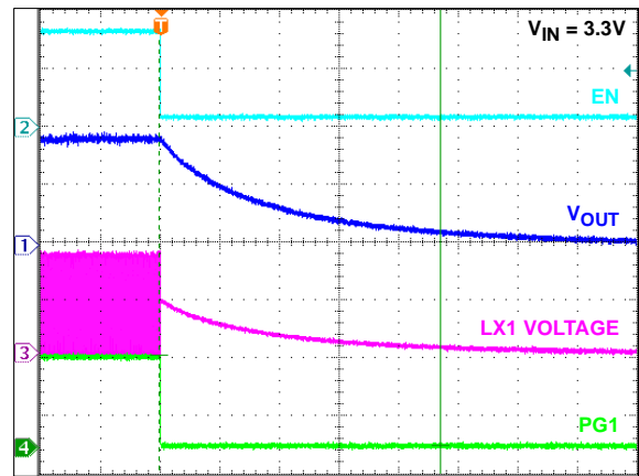
FIGURE 44. SOFT-DISCHARGE SHUTDOWN
