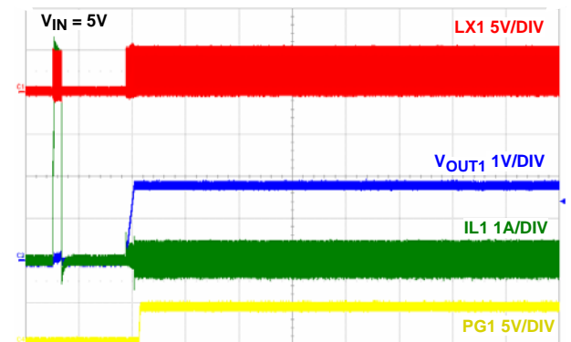
FIGURE 28. OUTPUT SHORT CIRCUIT RECOVERY (FROM HICCUP) CHANNEL 1
